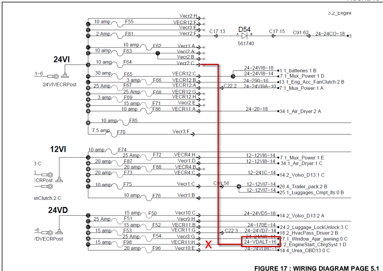
FIGURE 17 : WIRING DIAGRAM PAGE 5.1
