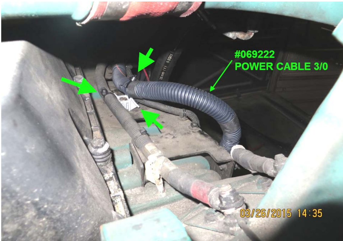
FIGURE 14: POWER CABLE ATTACHED TO #2 DOUBLE-TIE MOUNT AND PROPER NYLON TIES INSTALLATION
