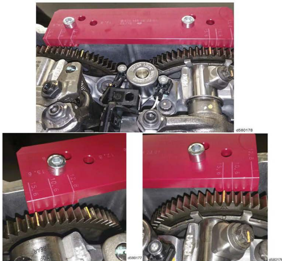
Figure 2. Comparing indicator marks on camshaft gears with indicator lines on timing plate. DD15/DD16 engine shown.
