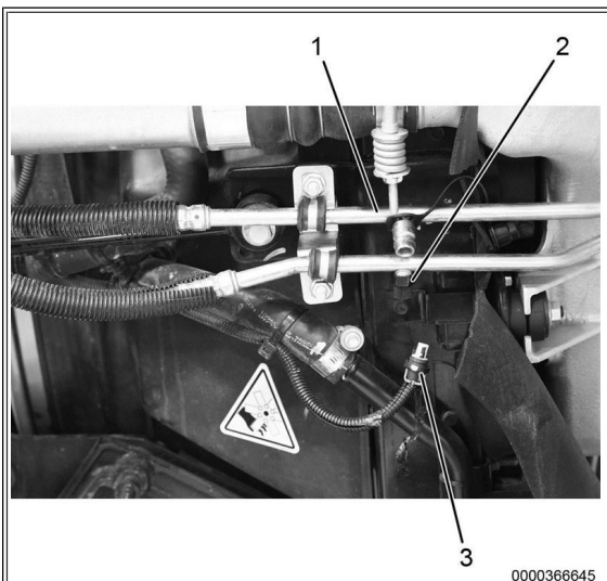
Figure 6: AC Compressor Discharge Line - N13 Equipped ProStar 122.
