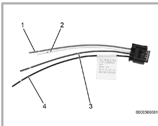
Figure 9: Pigtail
