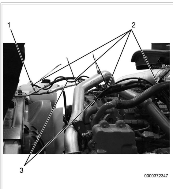
Figure 12: Kit-Supplied PT Sensor - Cummins Equipped ProStar 122.
