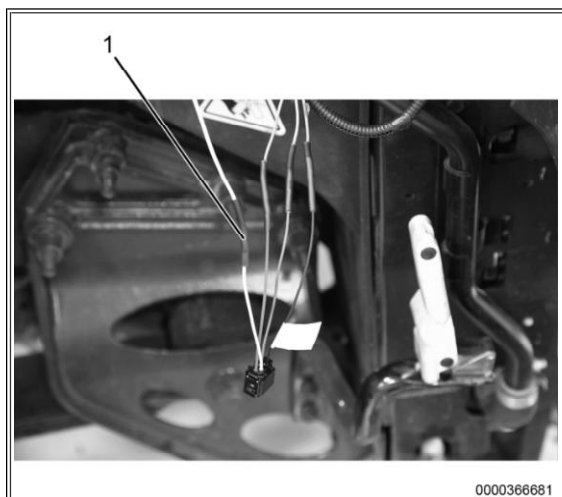
Figure 10: Pigtail Splice.
