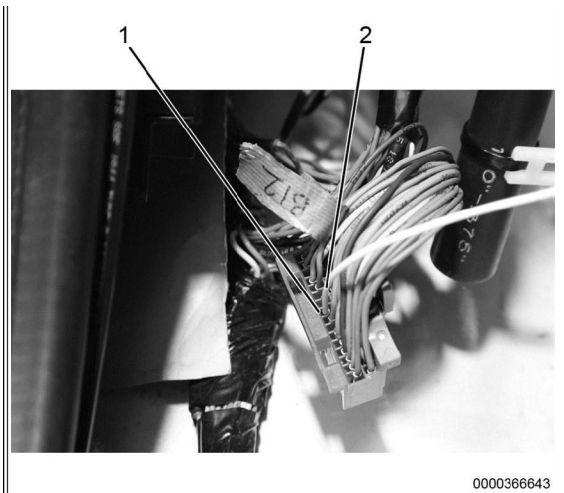
Figure 4: Cavity B9.
