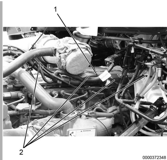
Figure 14: Kit-Supplied PT Sensor - Cummins Equipped ProStar 122.
