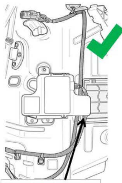
Correct Tow Harness Position to Right of BSD Bracket
