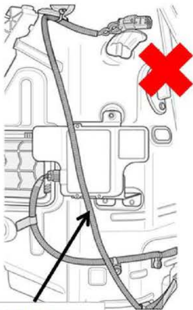
Incorrect Tow Harness Position over Top of BSD
