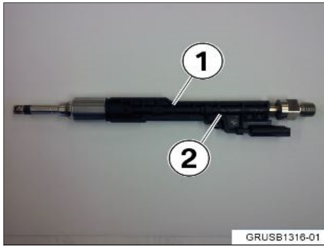
Bosch injector with black plastic housing (1). Injector part number location (2).
