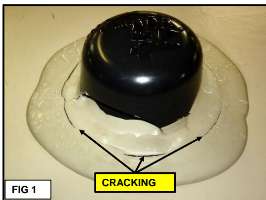
Fig 1-4: Inspect items mounted on the roof for signs of sealant cracking .
