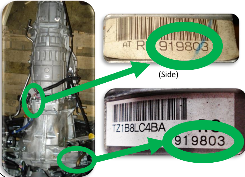
4AT & 5AT Serial Number Locations (Record only the 6 digits)
