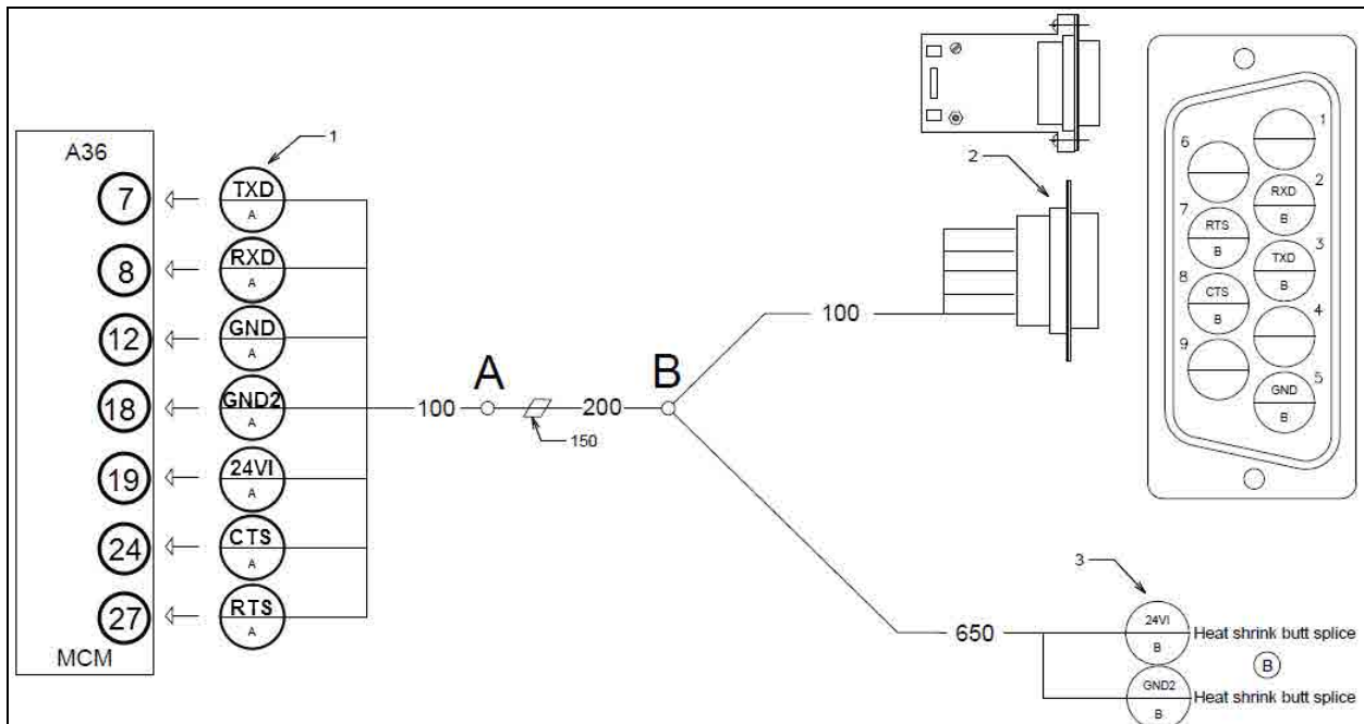
FIGURE 4: HARNESS 069420
