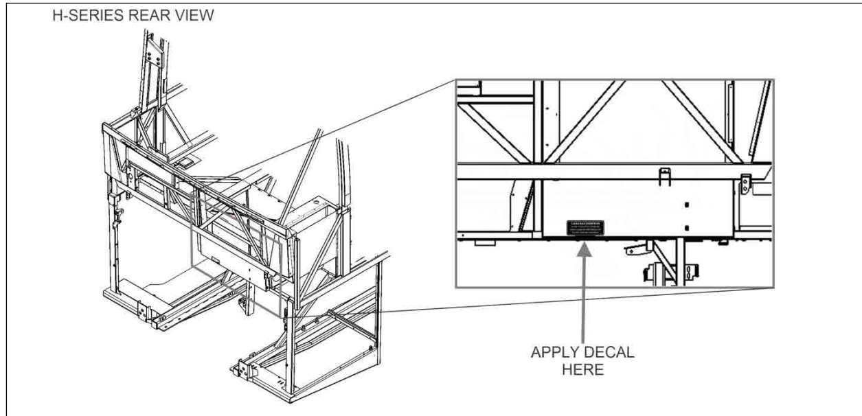
Figure 2 H-Series Structure, Rear View
