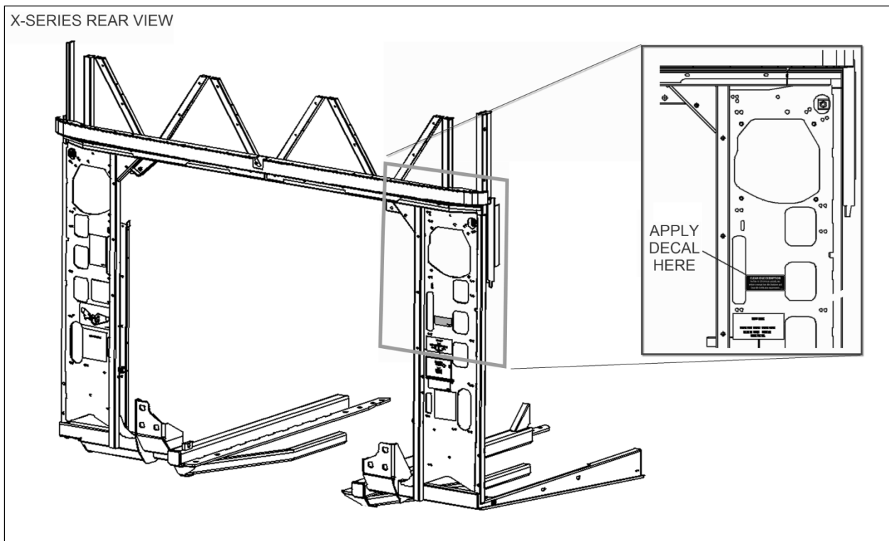
Figure 1 X Series Structure, Rear View
