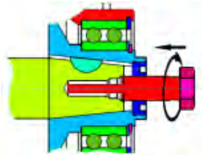
PULL OFF THE ROTOR WITH TOOL #7770159 (shown) or M16 BOLT
