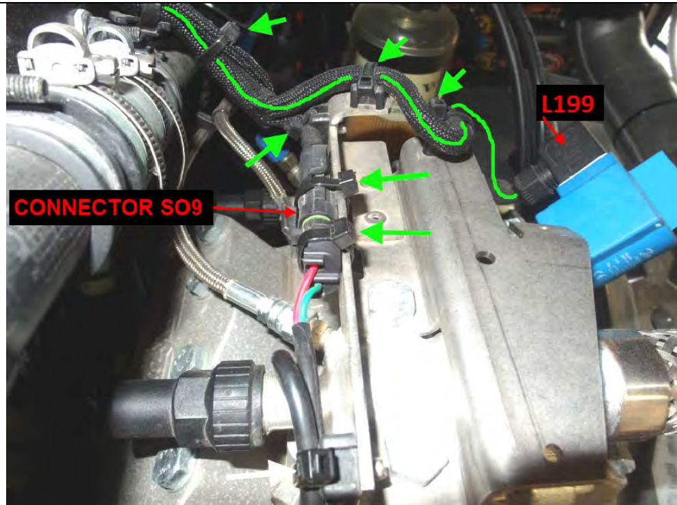
UNLOADER CABLE – NYLON TIES LOCATION SHOWN BY GREEN ARROWS ELECTROMAGNETIC CLUTCH CONNECTOR SECURED WITH TWO NYLON TIES FIGURE 29
