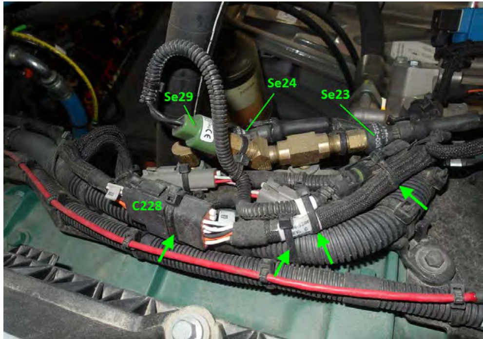
ATTACH THE EXCESS LENGTH OF CABLE ALONG MAIN STRAND OF HARNESS AS SHOWN- NYLON TIES LOCATION SHOWN BY ARROWS FIGURE 33
