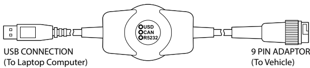
Figure 7, CANfox Adaptor Cable
