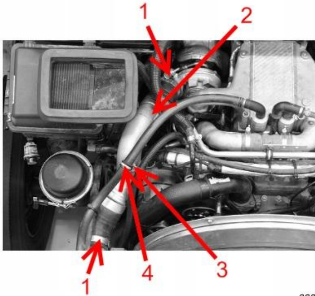
Figure 26: HPCAC Duct
