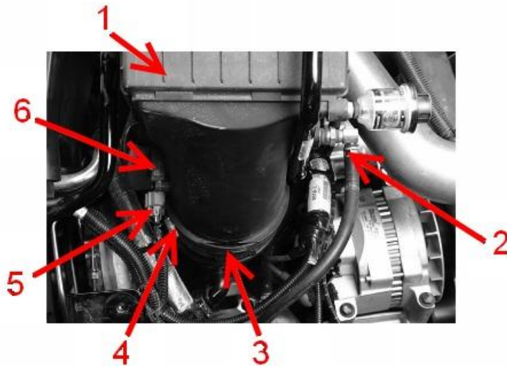
Figure 1: MAF Sensor and Air Compressor Inlet Hose.
