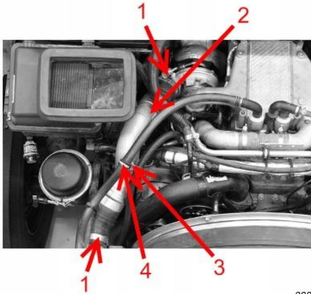
Figure 2: High Pressure Charge Air Cooler Duct
