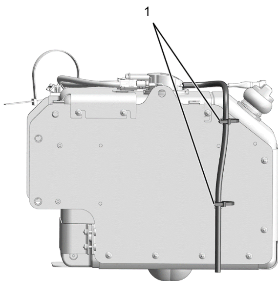
Figure 4. DEF Tank Vent Hose Routing – 15 Gal Tank
