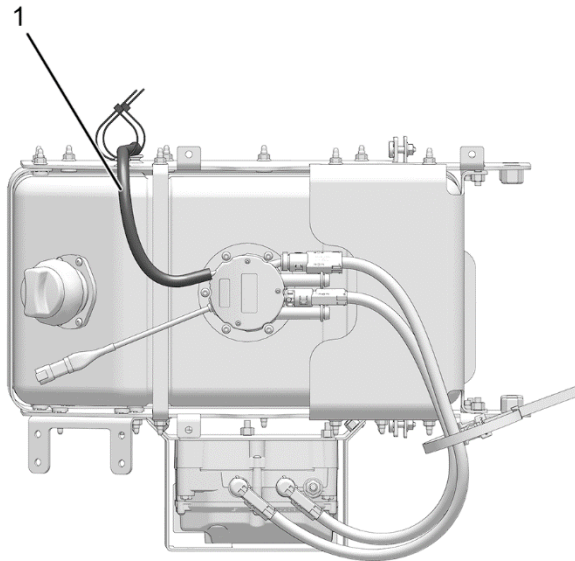
Figure 2. DEF Tank Vent Hose – 15 Gal Tank
