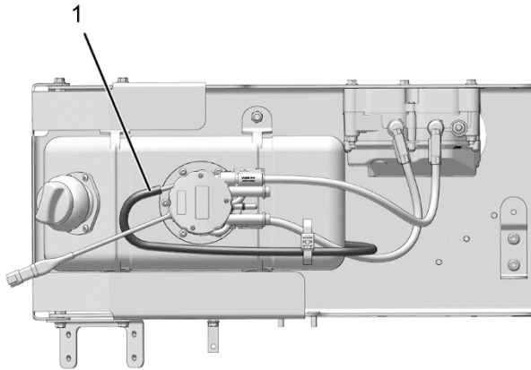
Figure 1. DEF Tank Vent Hose – 5 Gal Tank
