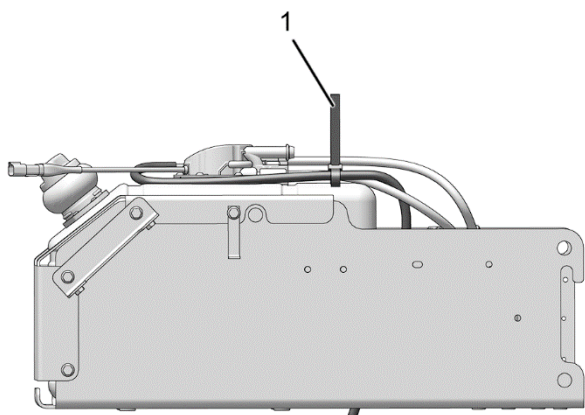
Figure 3. DEF Tank Vent Hose Routing – 5 Gal Tank
