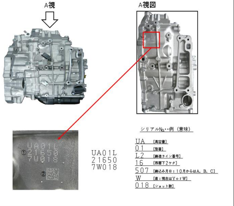
Figure 1: Transmission serial number location for UA80 from AW (left) and Kinuura (right)
