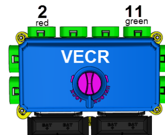
FIGURE 10 : VECR
