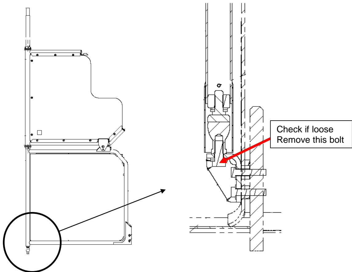
Figure 1: Affected bolt location
