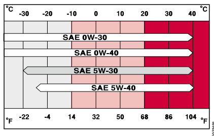
Viscosity chart
