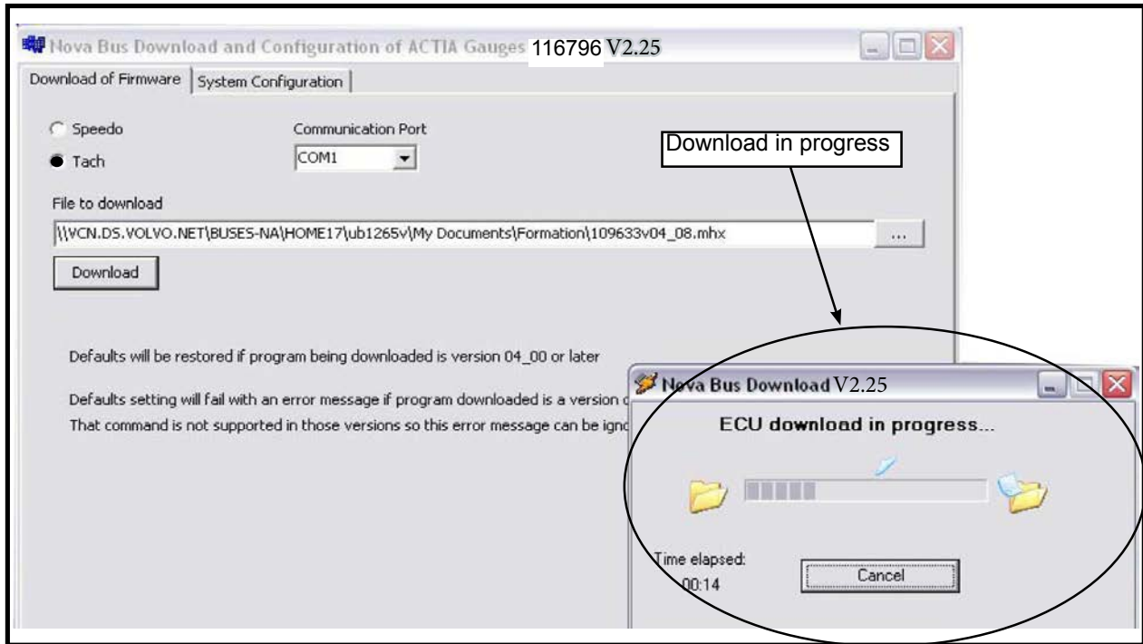
Figure 29 - Program Download
