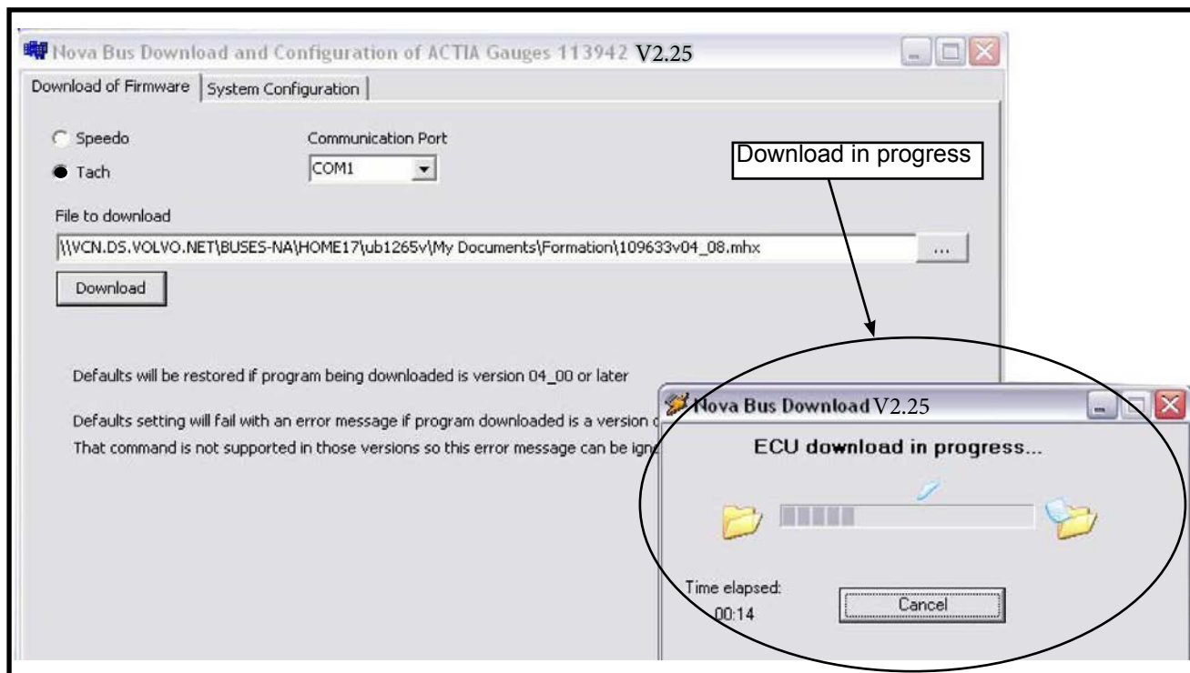
Figure 38 - Program Download
