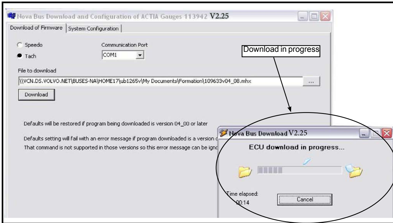
Figure 35 - Program Download
