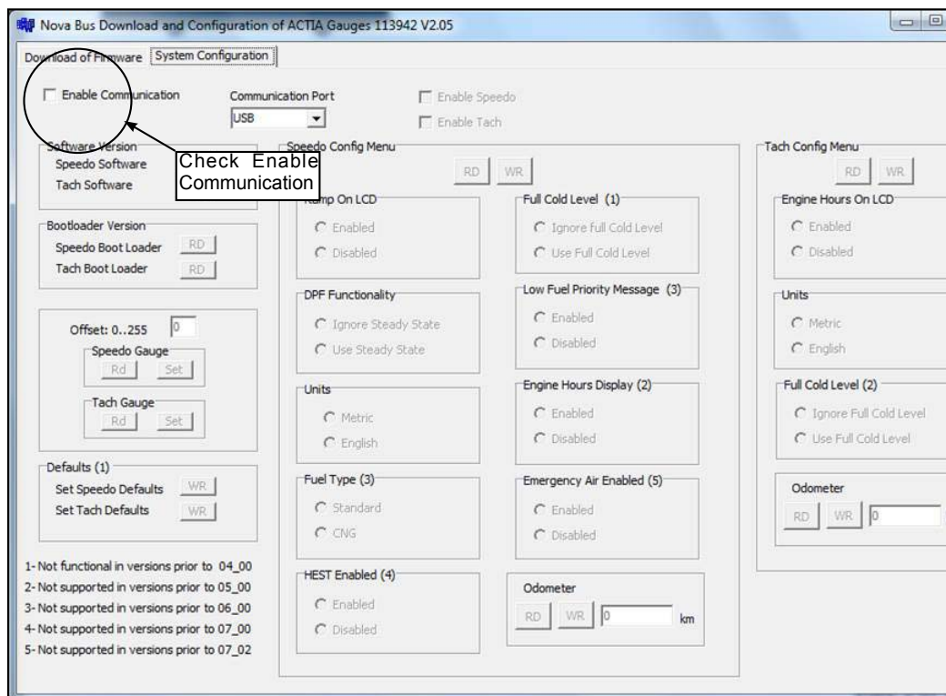
Figure 10 - Enable Communication
