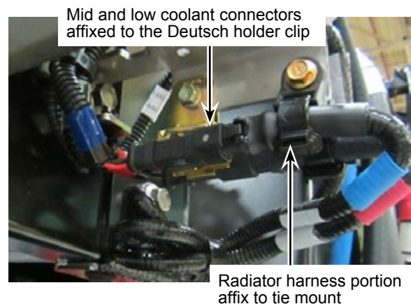
Figure 4 - Installation of Harnesses to the Support Bracket
