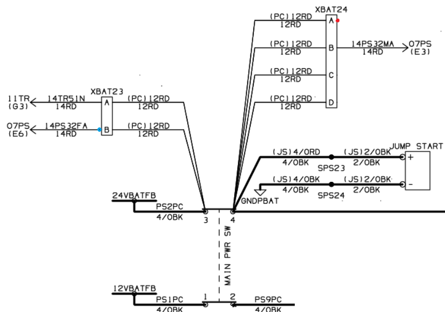
Figure 3: Electrical schematic
