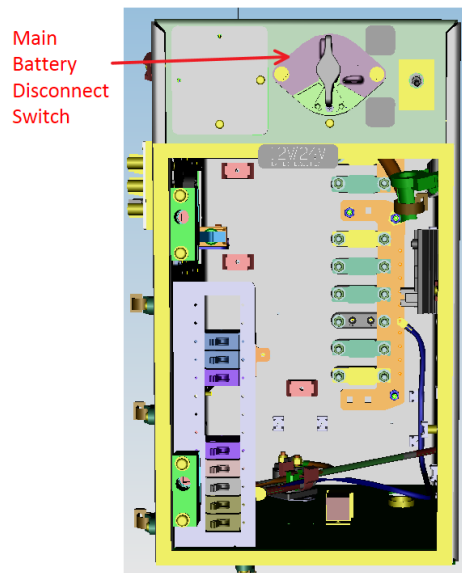
Figure 2: Fuse box main battery disconnect switch
