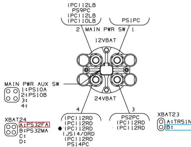
Figure 2: Battery disconnect switch wiring diagram
