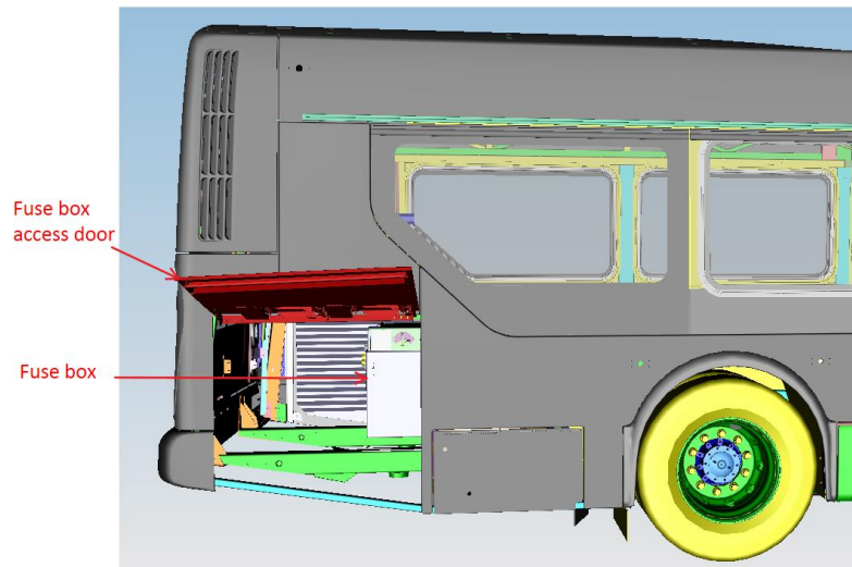
Figure 1: Fuse box location (curb side view)
