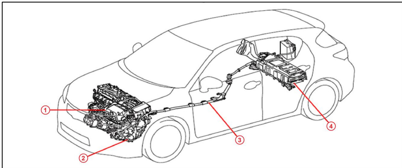
Figure 1. High-Voltage Components and Cables
