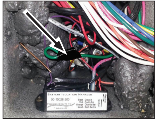
Figure 2 - Battery Isolator Wiring After Correction
