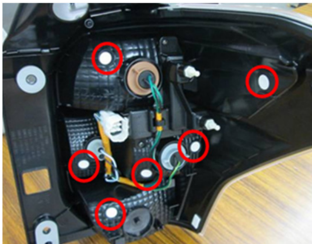
Rear view of the new combination lamp showing the 6 additional breathing holes.
