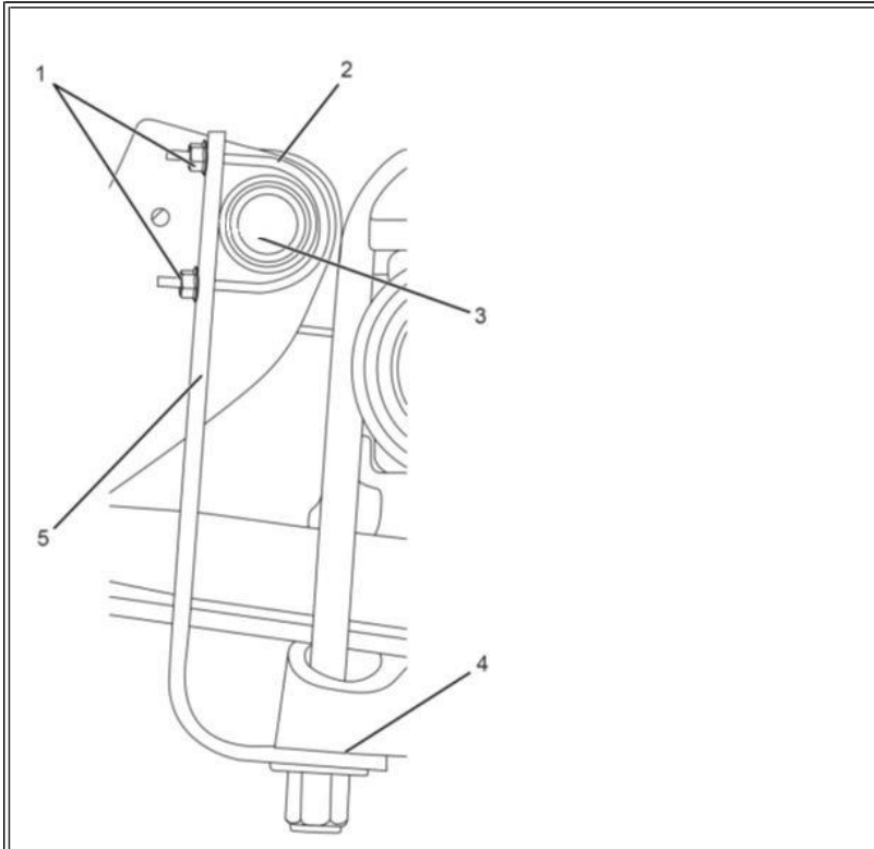
Figure # 2: Support Bracket
