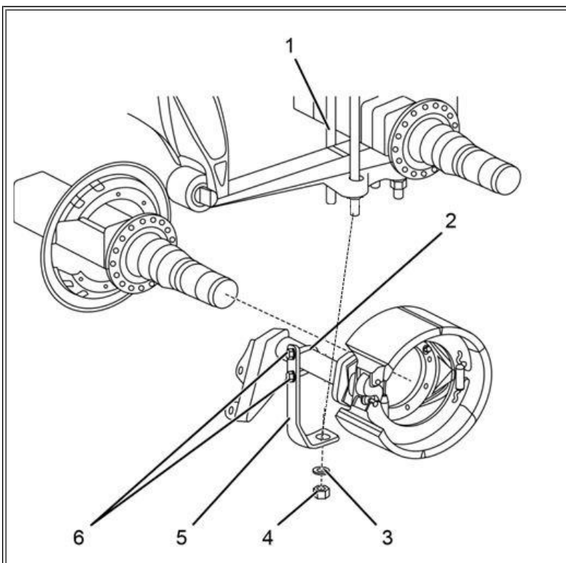
Figure #1: Cam Tube
