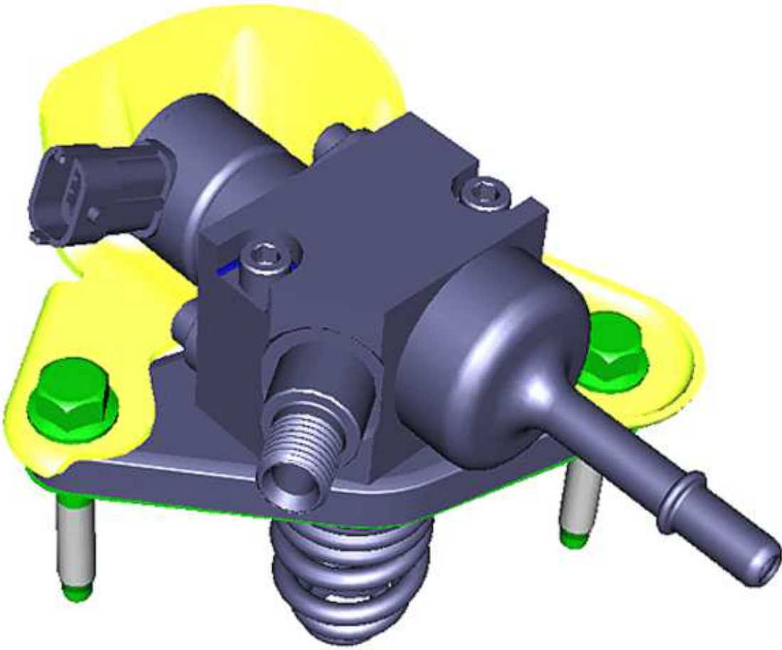
Stanadyne style fuel pump part number 12669519 and fuel pipe part number 12673077 as shown above.
