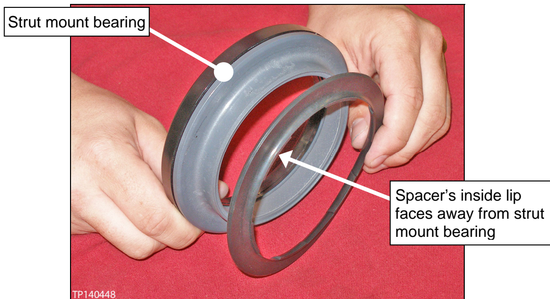
Direction of spacer installation
