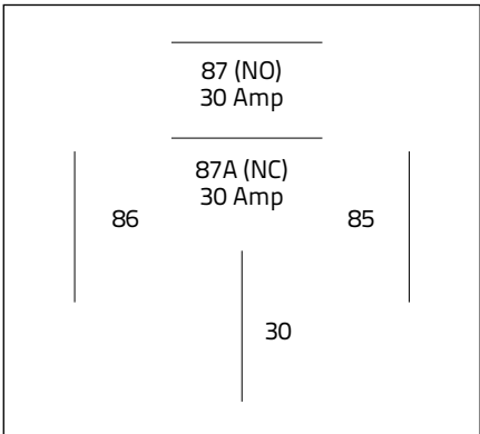
Terminal Connection
