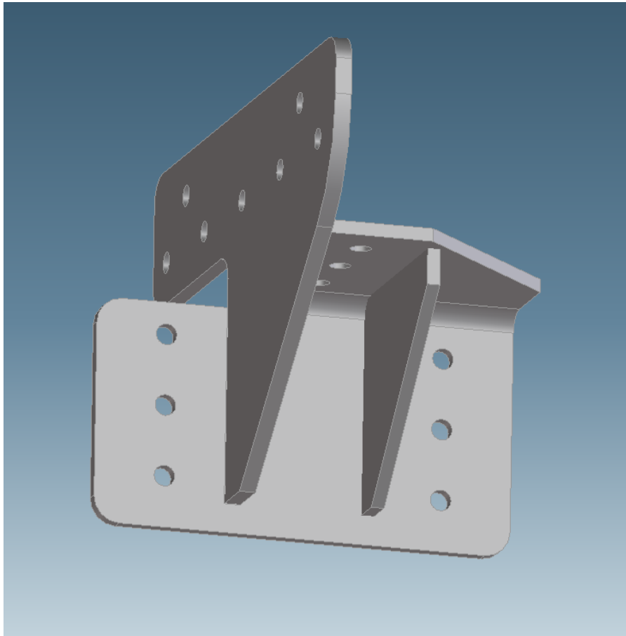
Attaching Gusset #17-05279-100 and -200
