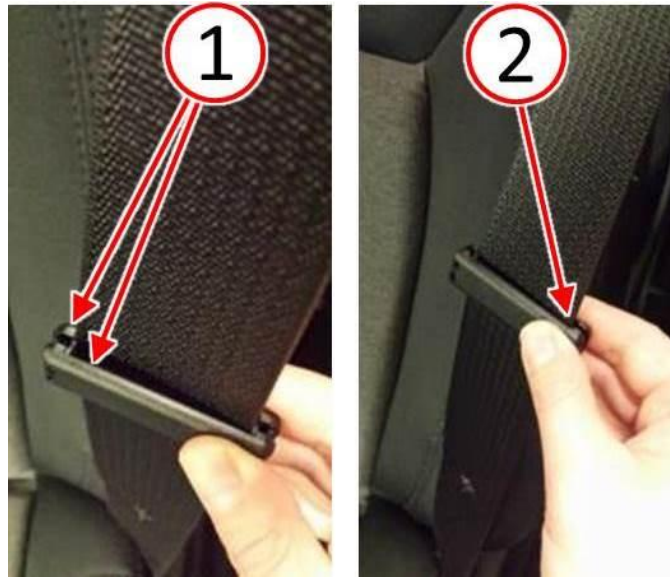
Fig. 4 Press Comfort Clip Halves Together To Fasten
