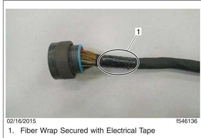
Fig. 15, Fiber Wrap Secured with Electrical Tape
