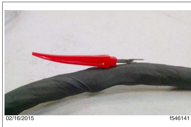
Fig. 10, Cutting the Fiber Using the Blunt End of the Seam Cutter
