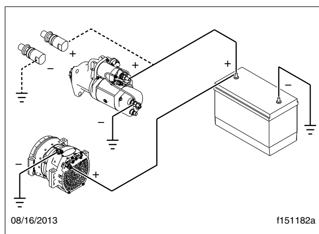
Fig. 2, EPA07: the alternator does not route through the starter. Use "Starter Path Check — EPA07 Engines" for Check 5, unless the vehicle has jump posts.
