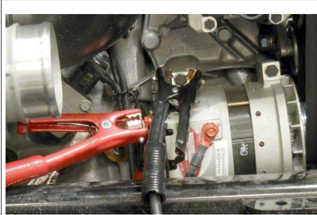
Fig. 7, For EPA10 and EPA04 engines, the starter path can be checked by loading the circuit at the alternator.
