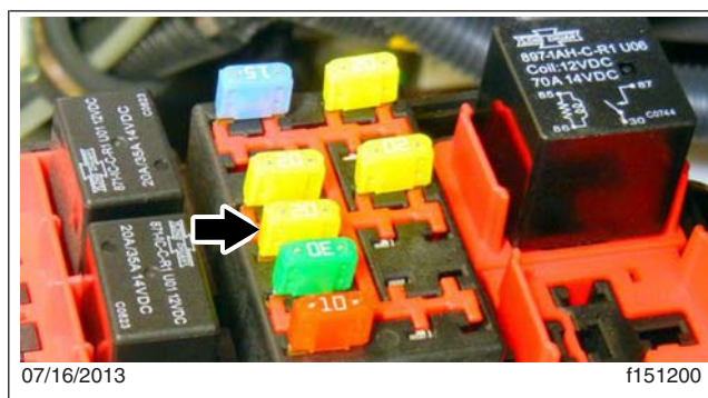
Fig. 16, EPA07 vehicles: 20 amp remote sense fuse, location F7 in the Powertrain PowerNet Distribution Module (PTPDM).
