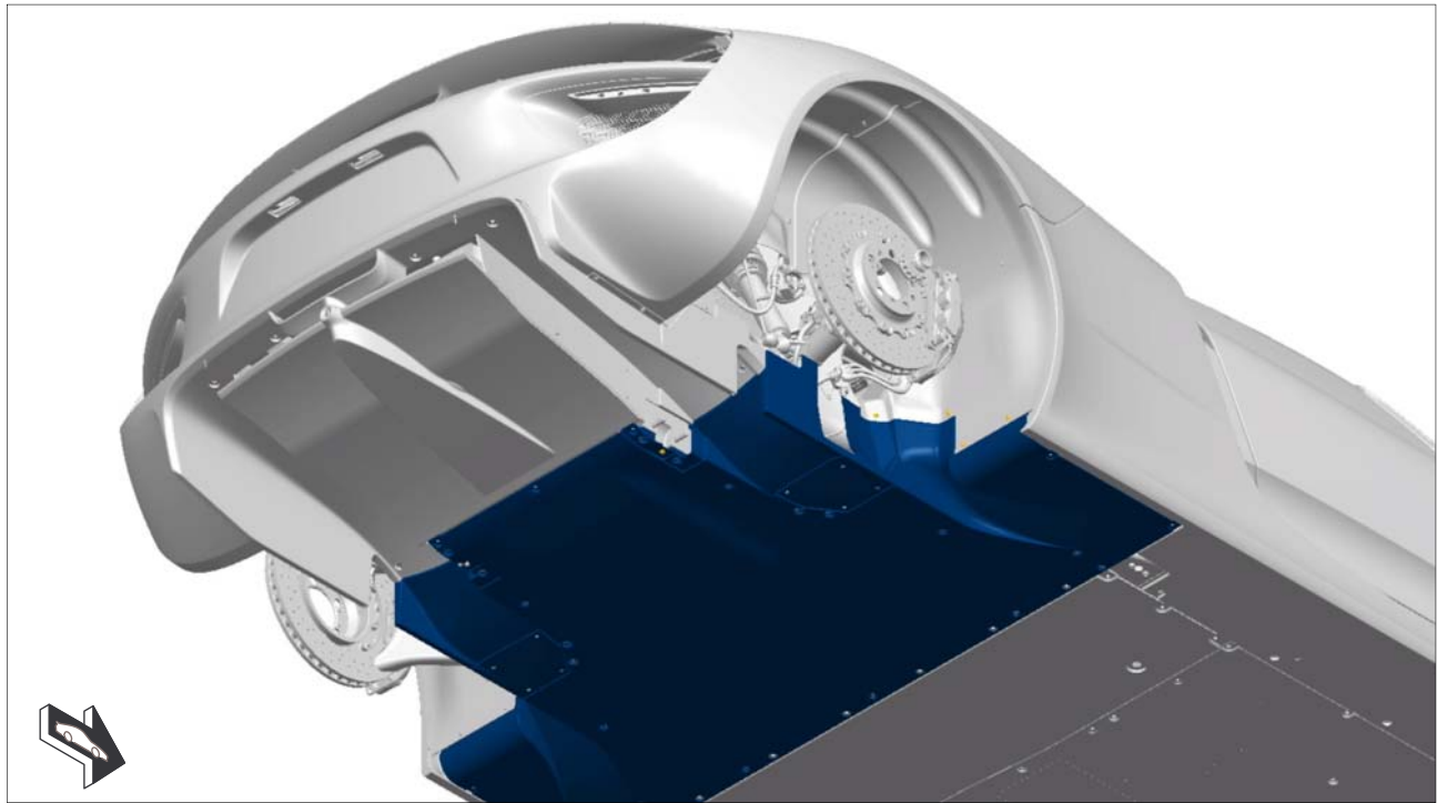
Installation position of rear underbody panelling
