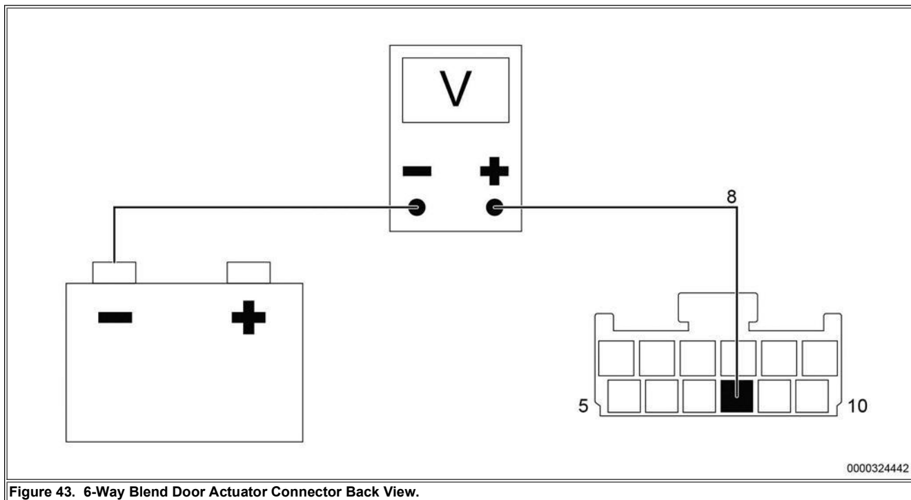
Figure 43. 6-Way Blend Door Actuator Connector Back View.
