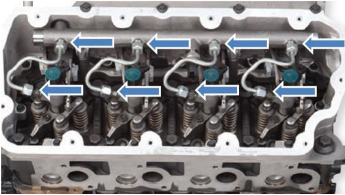
Figure 2: Injector Jumper Tube Leak Locations
