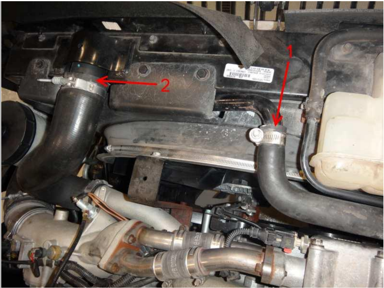
Figure 27: Dearation Tank Assembly
