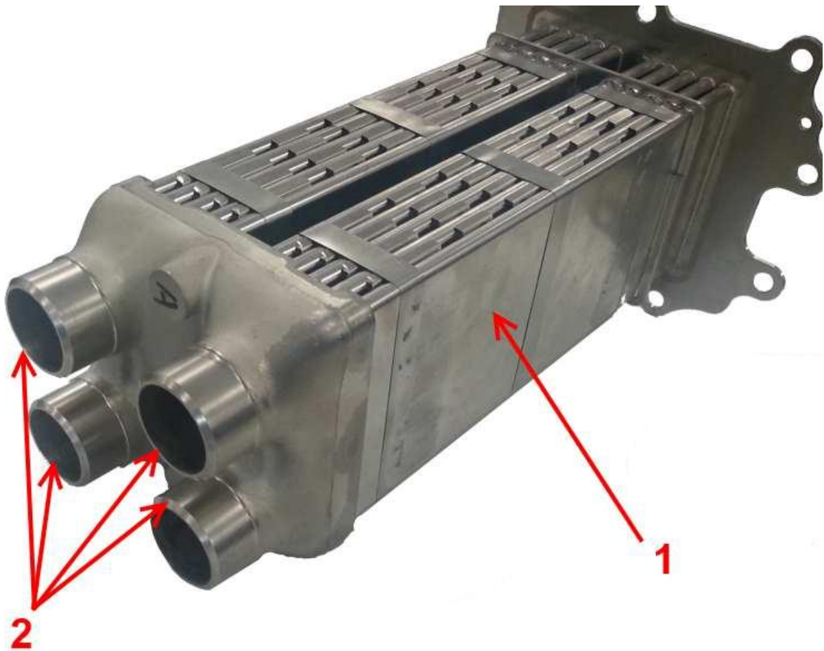
Figure 16: Low Temp Cooler Inlet Manifold
