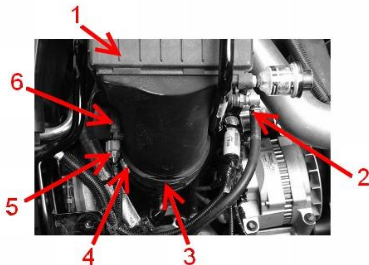
Figure 1: MAF Sensor and Air Compressor Inlet Hose.
