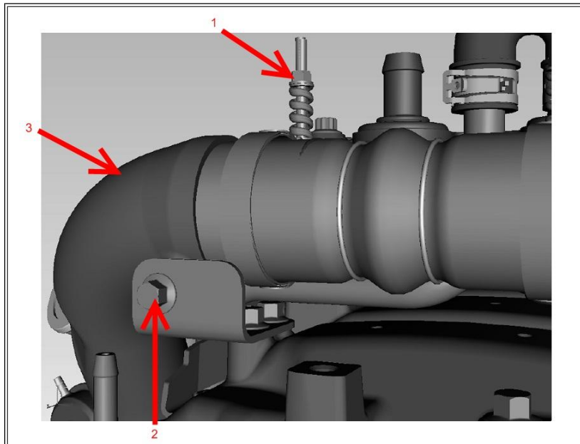
Figure 2: Interstage Tube Removal
