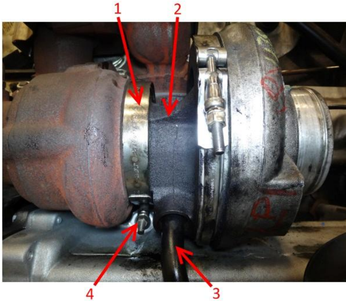
Figure 3: Oil Supply Tube at Oil Cooler Housing
