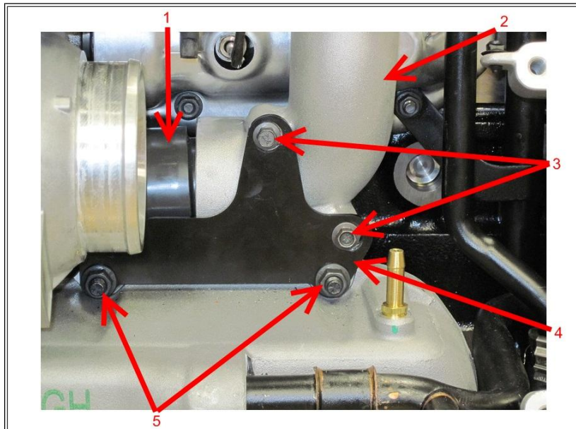
Figure 9: Oil Supply Tube at Oil Cooler Housing
