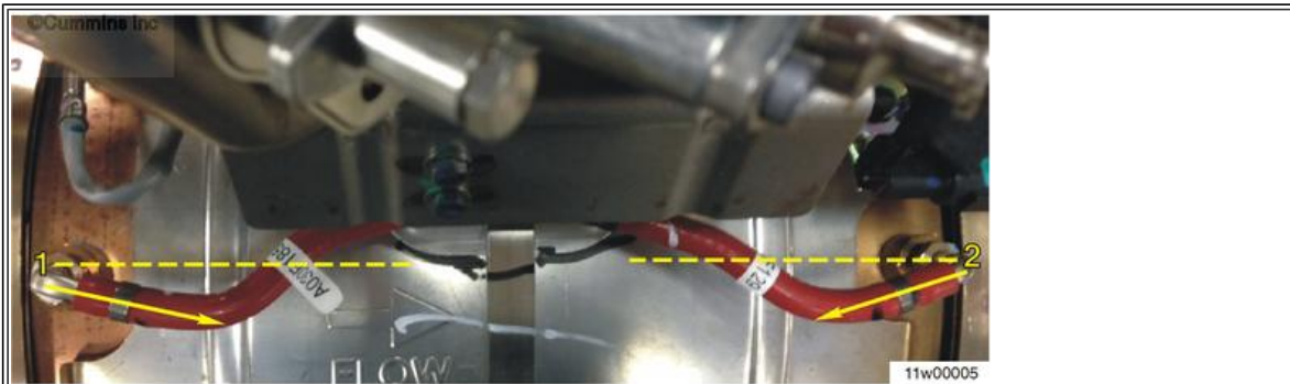
Figure 1: Incorrect DPF differential pressure sensor orientation
