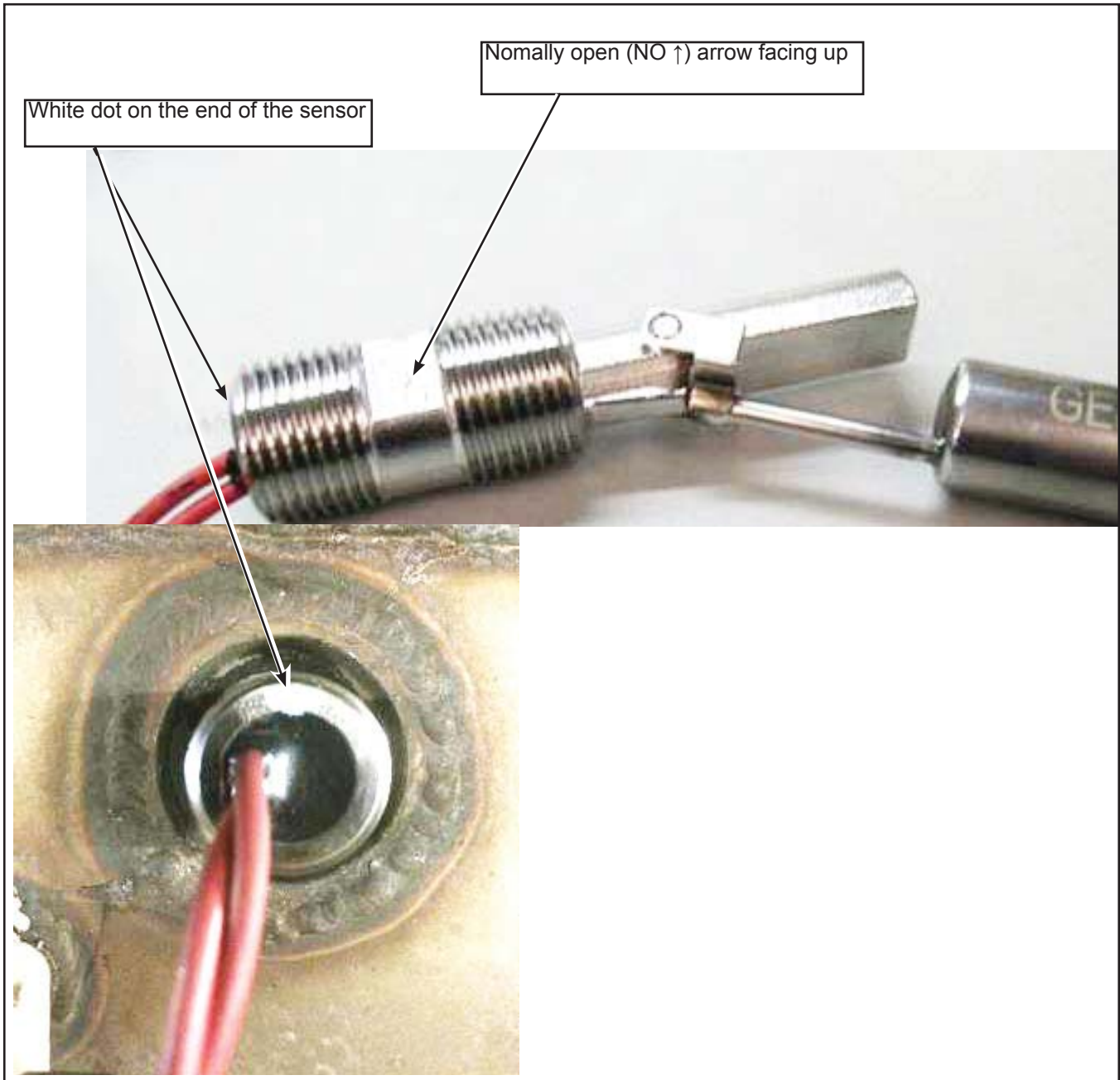
Figure 2 - Low Coolant Level Sensor Position
