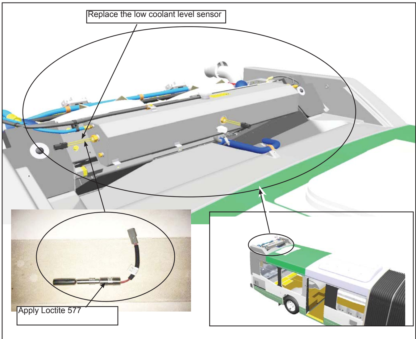
Figure 1 - Replace the Low Coolant Level Sensor
