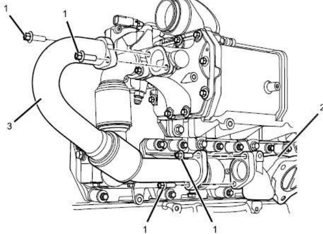
Figure 2: Outboard EGR Inlet Tube
