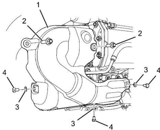
Figure 1: Heat Shield (Cylinders 4 - 6)
