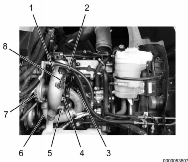
Figure 18: HP and LP Turbocharger Connections
