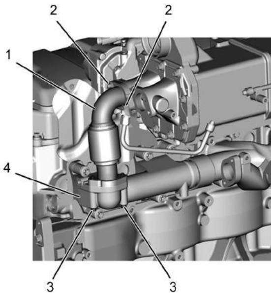
Figure 3: Inboard EGR Inlet Tube
