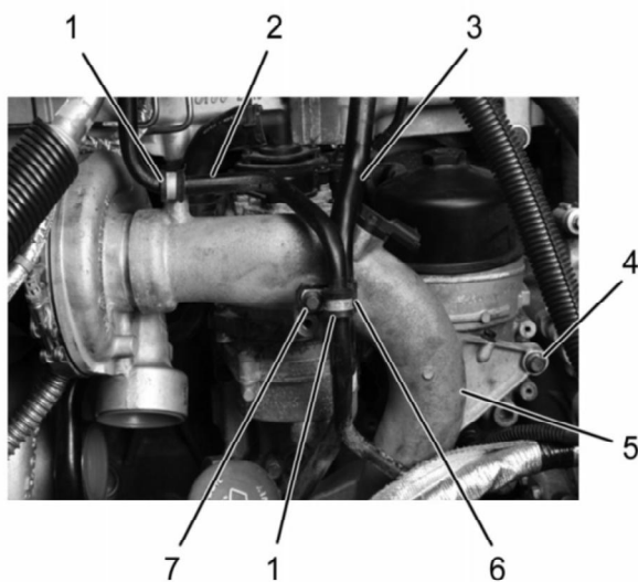
Figure 19: Coolant Supply Tubes
