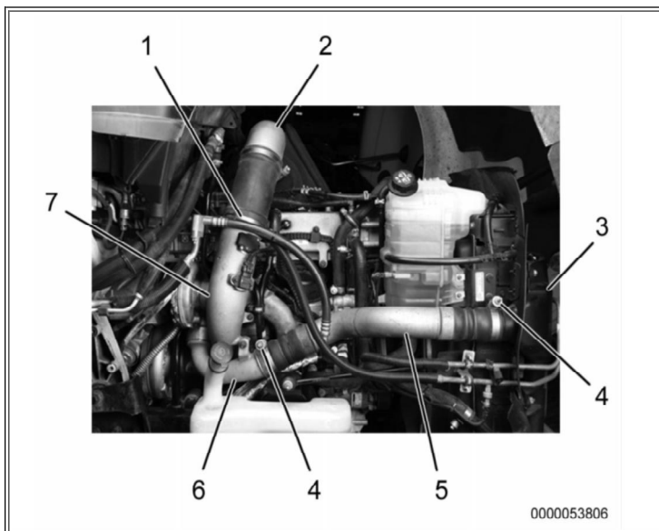
Figure 17: HP Turbocharger Connections
