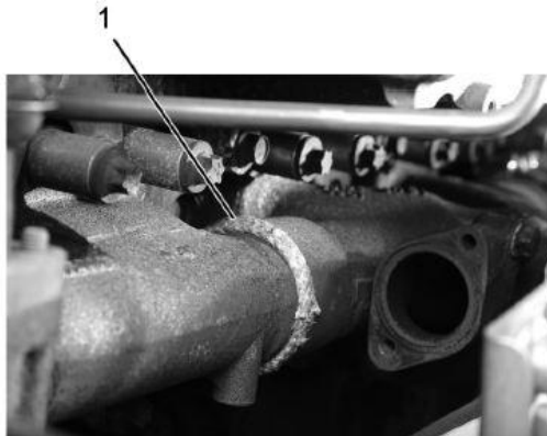
Figure 9: Rear Exhaust Manifold Ring Seal Packing
