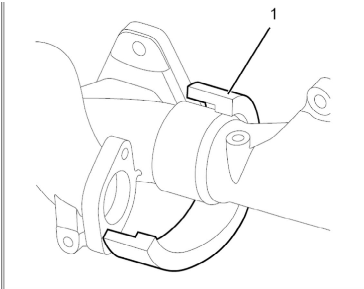
Figure 27: Front Exhaust Manifold Ring Seal Ceramic Mat Wrap Item 1: Ceramic mat wrap
