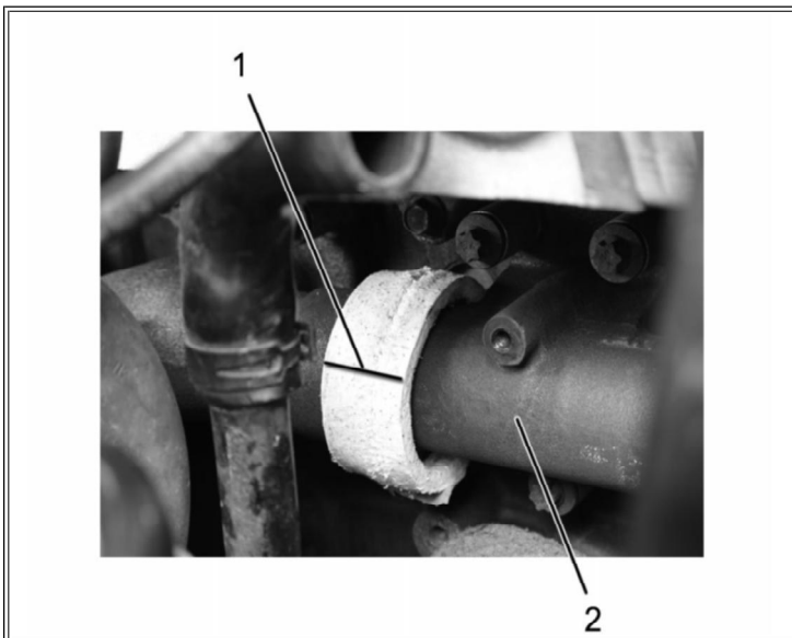
Figure 28: Front Exhaust Manifold Ring Seal Ceramic Mat Wrap Alignment Item 1: Ceramic mat wrap join Item 2: Manifold midpoint
