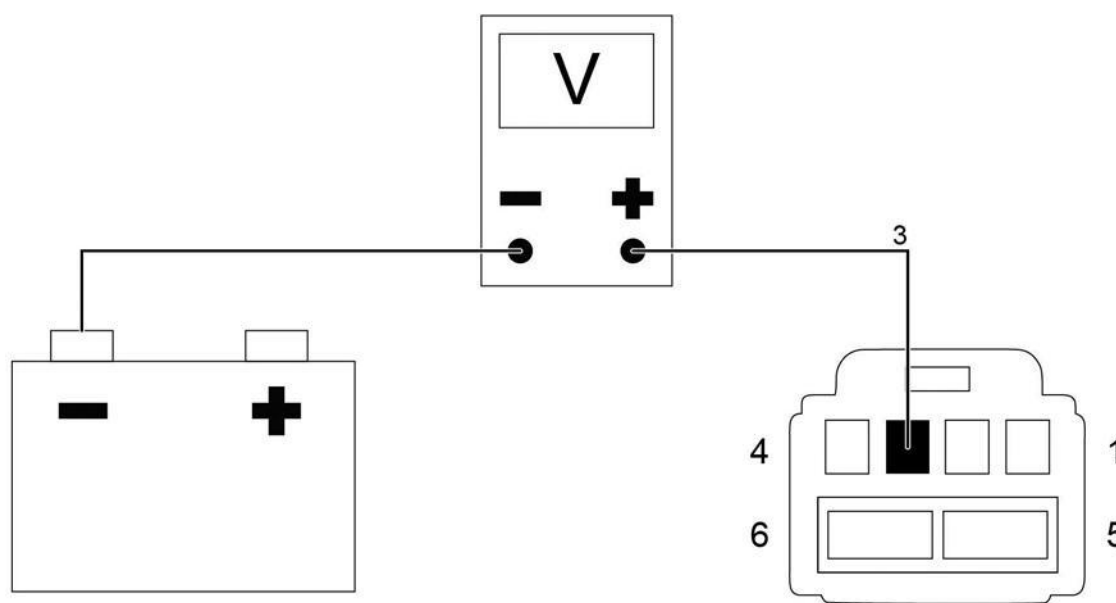
Figure 31. 6-Way LPM Connector Back View.
