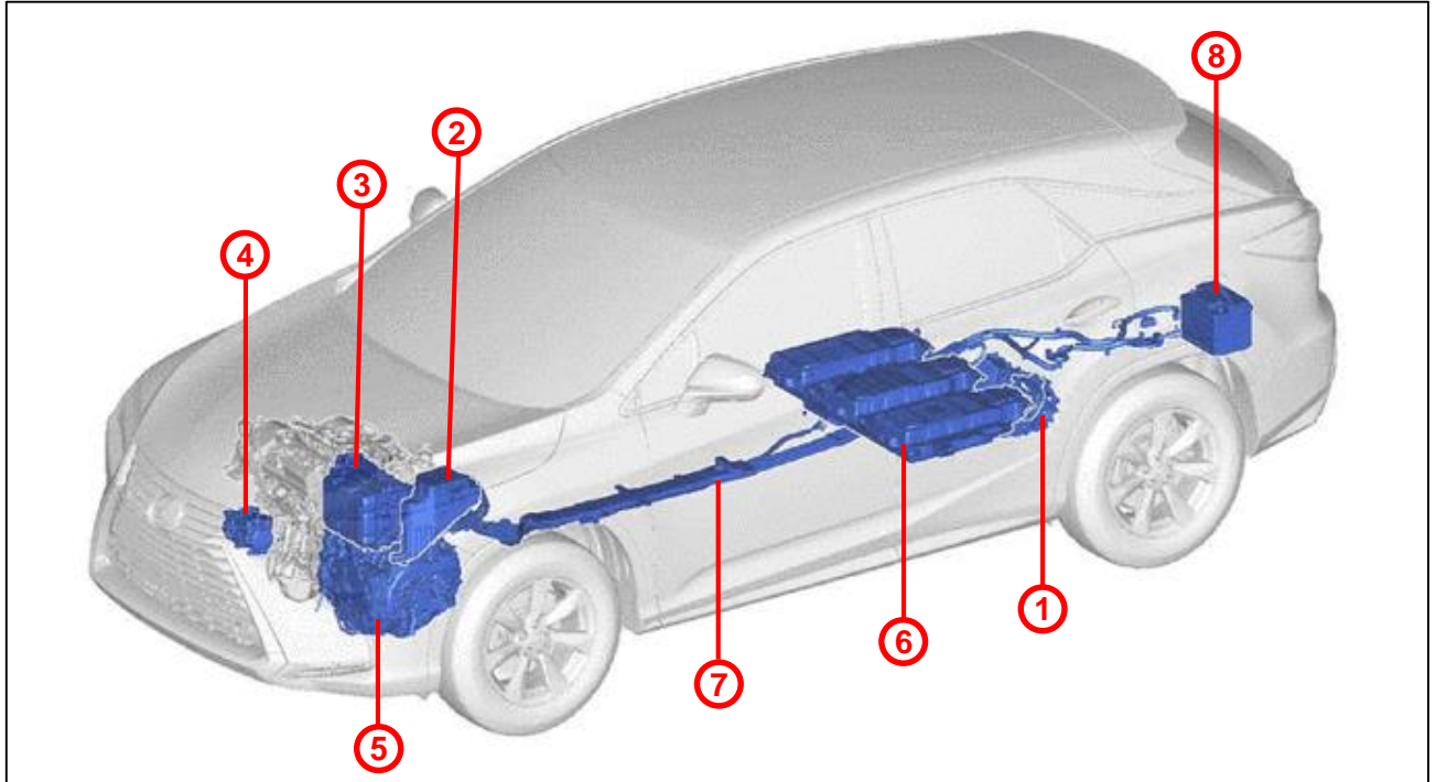
Figure 1. High-Voltage Components and Cables
