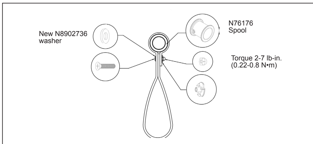
Figure 5 - Strap Torque
