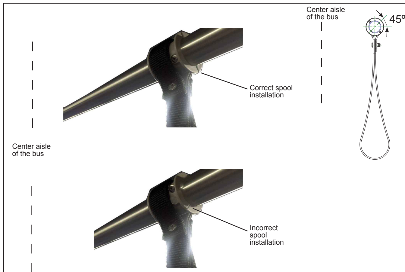
Figure 1 - Spool Installation
