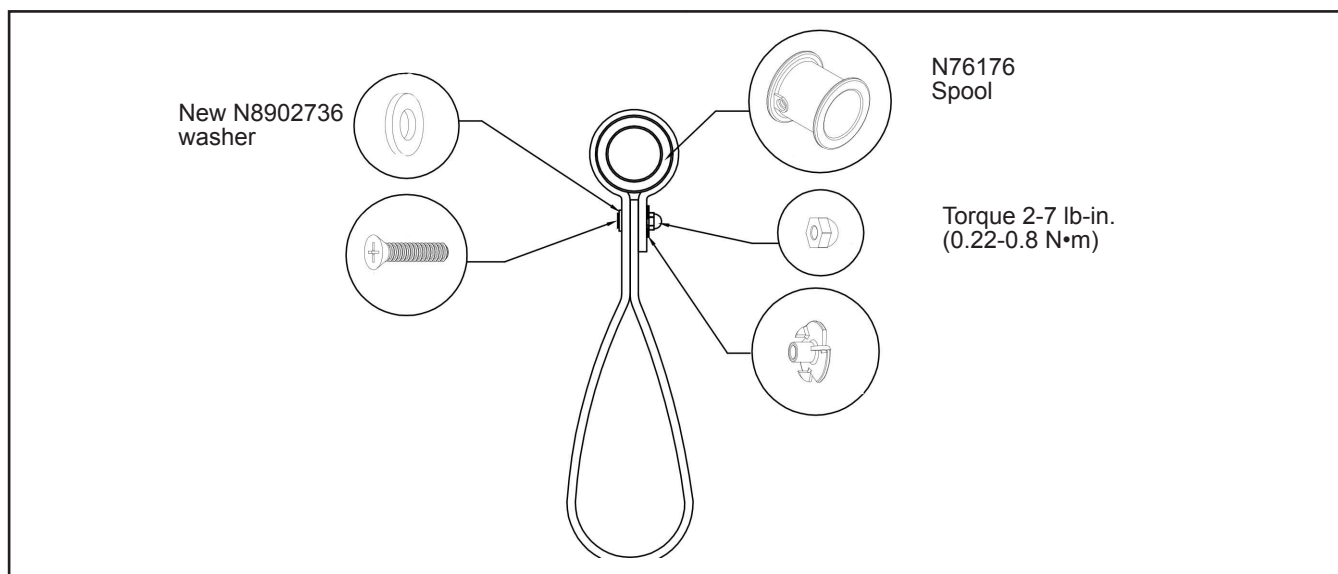
Figure 3 - Strap Assembly
