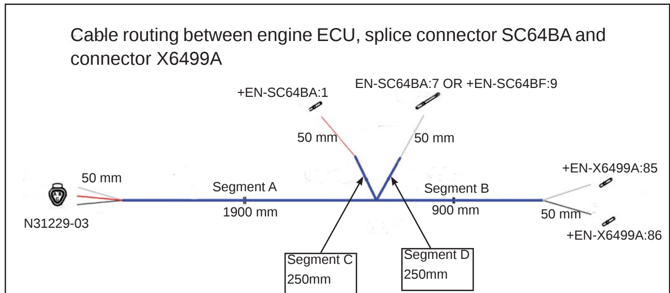
Figure 1 - Replacement Cable N80191
