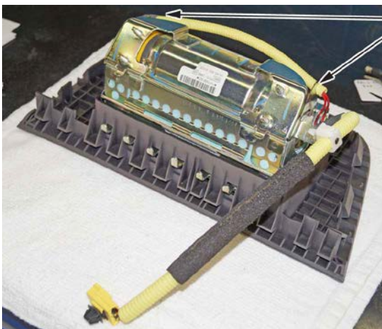
INFLATOR BRACKETS
