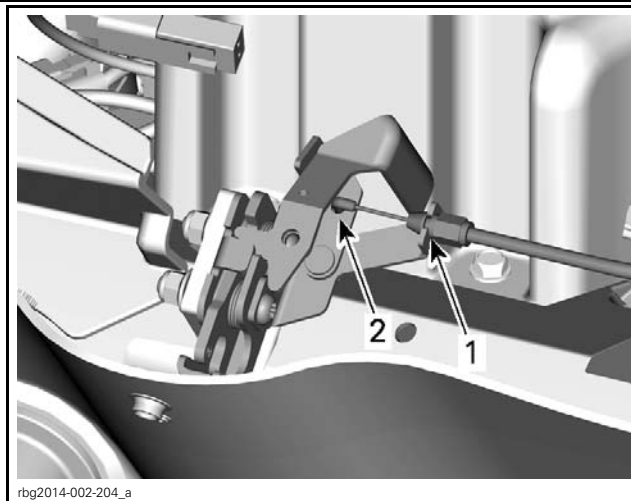
STORAGE COMPARTMENT LATCH (RT MODEL) 1. Cable retainer 2. Latch pivot plate
