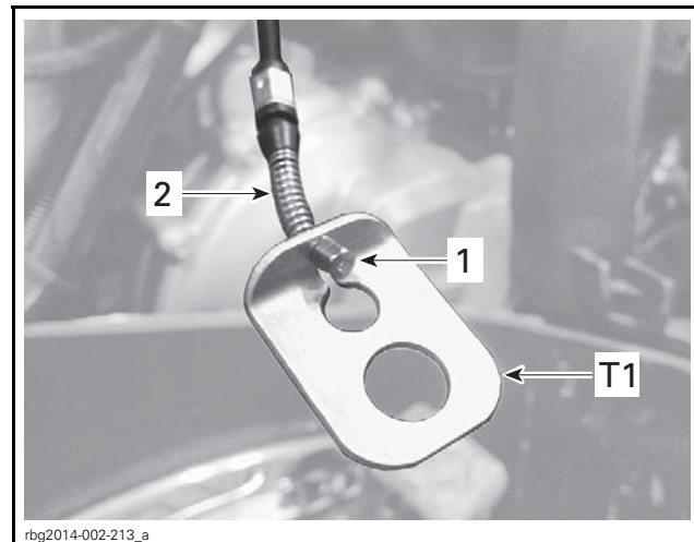
RS AND ST MODELS 1. Cable end 2. Spring
