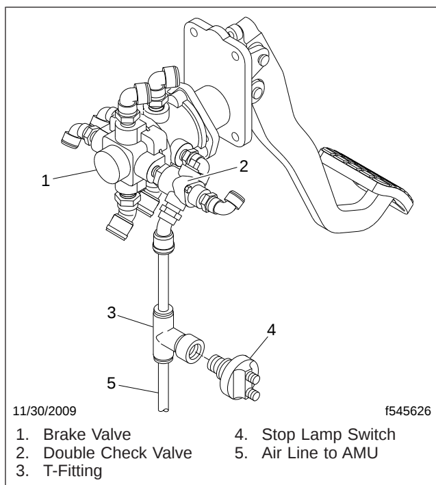
Fig. 1, Stop Lamp Pressure Switch Installation
