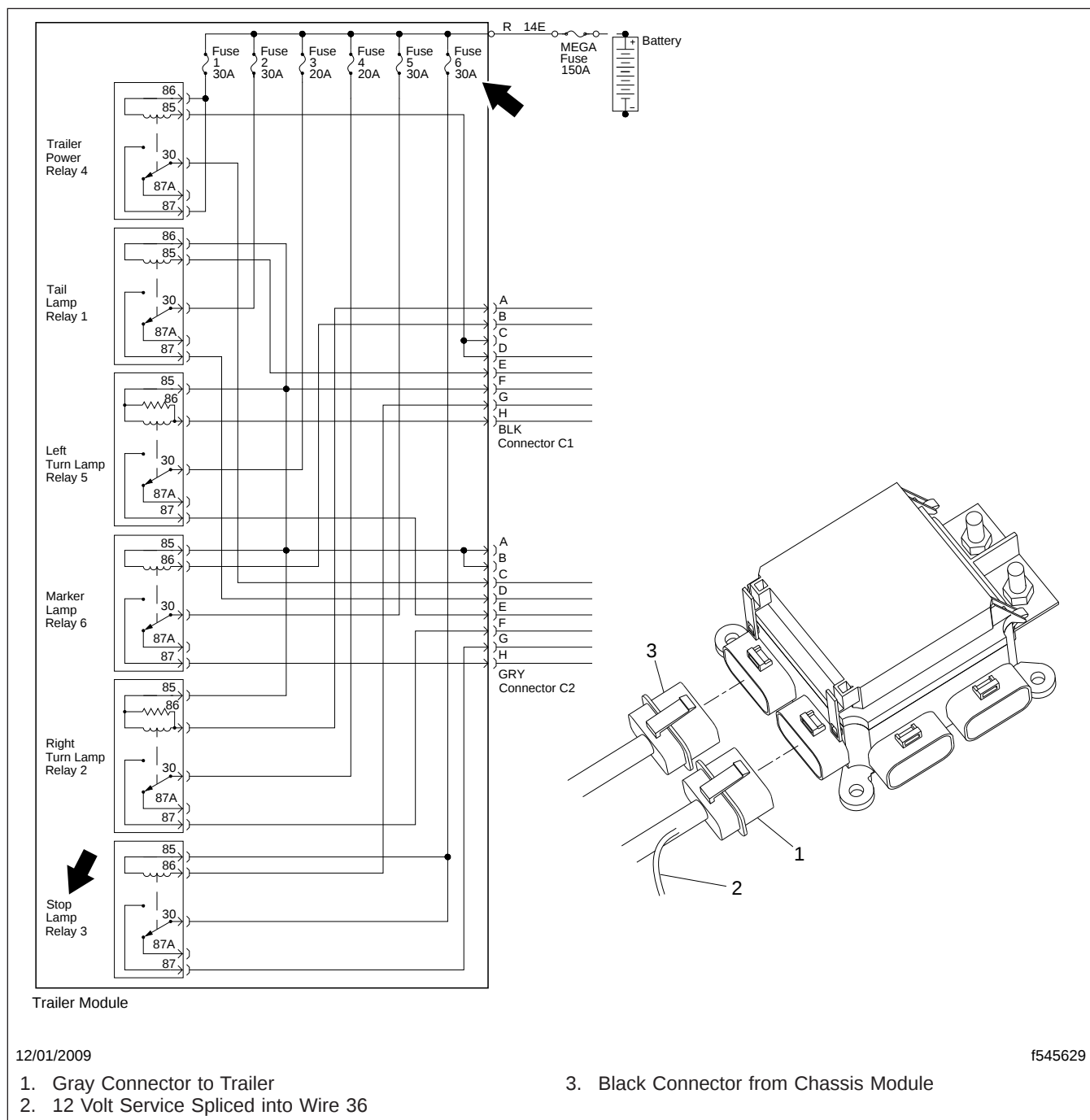
Fig. 4, Stop Lamp Signal Access at the Trailer PDM
