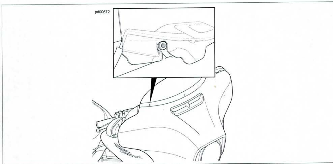
Figure 2. Windshield/Wind Deflector Keyhole
